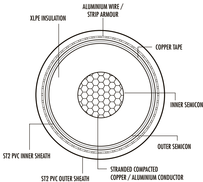
TYPICAL CONSTRUCTION OF POLYTAB 1 CORE HT XLPE CABLE
