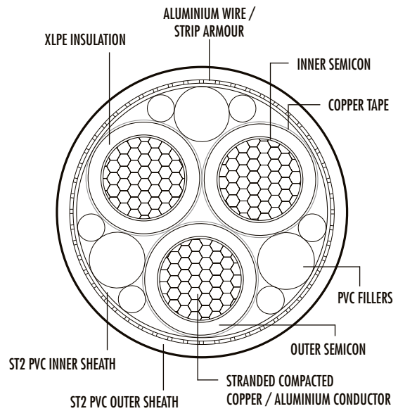
TYPICAL CONSTRUCTION OF POLYTAB 3 CORE HT XLPE CABLE
